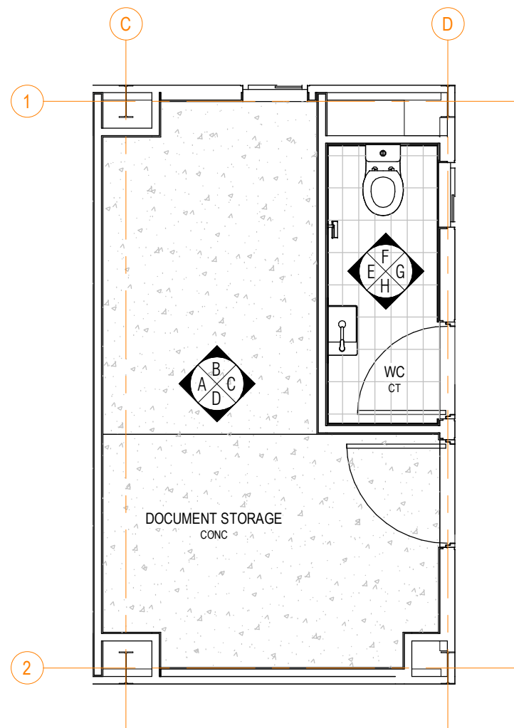
DOCUMENT STORAGE AND TOILET KEY PLAN SCALE : 1 : 50
